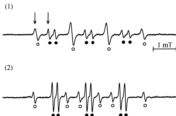
Fig. 1. (1) EPR spectrum obtained after UV-photolysis in the aqueous solution of hydrogen peroxide, DMPO, and PBN: (○) \bullet DMPO-OH ( g = 2.0059 ) and (●) \bullet PBN-OH ( g = 2.0057 ). (2) EPR spectrum obtained after UV-photolysis in the benzene solution of tetraphenyllead, DMPO, and PBN: (○) \bullet DMPO-Ph ( g = 2.0045 ) and (●) \bullet PBN-Ph ( g = 2.0054 ). Peaks marked with arrows were used to determine the concentration of spin adducts.
